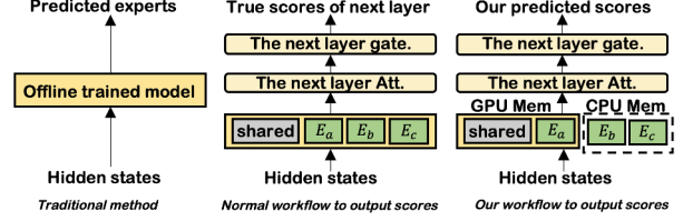
Fig. 8: Our prefetching method compared to traditional method and normal workflow to output true scores.
