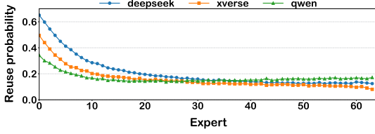
Fig. 7: The reuse probability of experts based on score (in descending order) in three MoE models.
