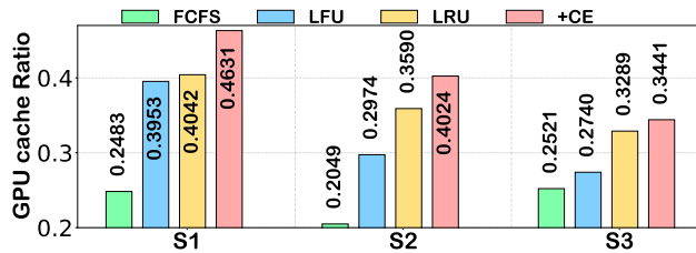
Fig. 19: “+CE” vs traditional cache methods.
