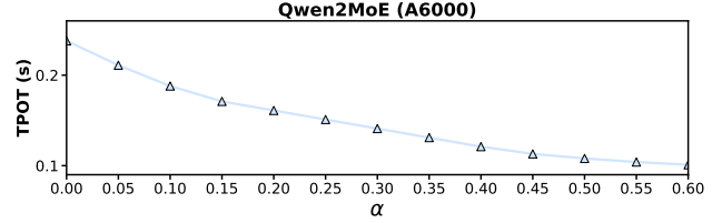
Fig. 11: Relationship between \alpha and T(\alpha) .
