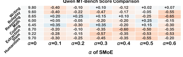
Fig. 15: Per-domain Analysis of SMOE.
