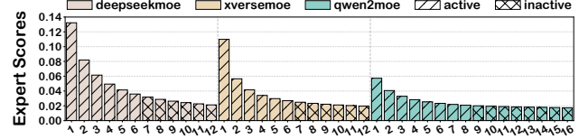
Fig. 5: Average scores at each ranked position across all tokens and layers (sorted in descending order) from 100 prompts.
