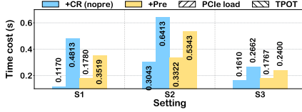
Fig. 20: PCIe time vs TPOT.
