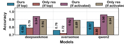
Fig. 21: Prefetching accuracy.
