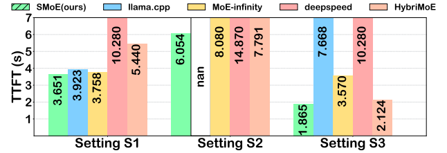
Fig. 16: Prefilling time of baselines and SMOE on average.
