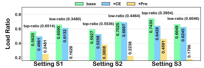
Fig. 18: Fewer top/low-score experts loading.
